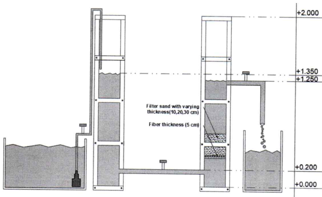
Fig. 1 The simulation equipment of the filtration process
