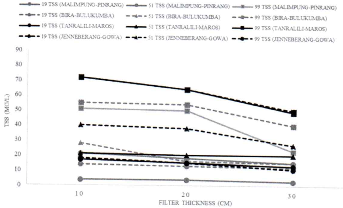
Fig. 5 Effect of filter thickness on TSS reduction
